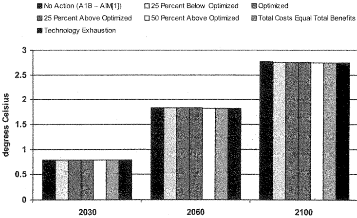
3 Figure 2.5-4 Increase in Global Mean Surface Temperature for the A1B Scenario and 4 MY 2011-2015 Standard and Potential MY 2016-2020 5
