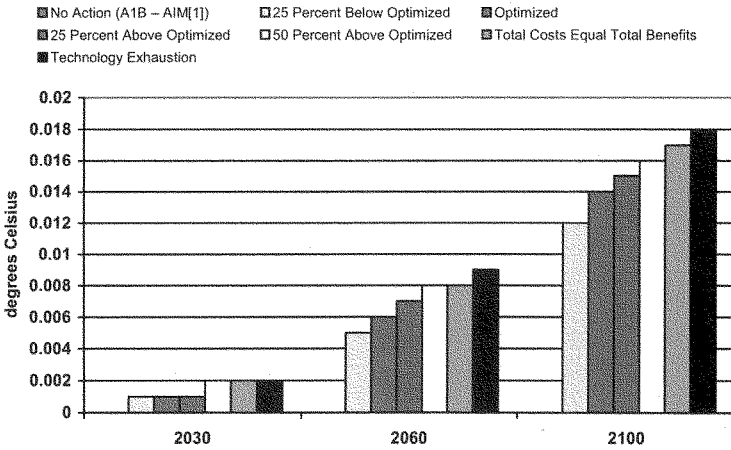
3 Figure 2.5-6 Reduction in the Growth of Global Mean Temperature for the A1B Scenario 4 MY 2011-2015 Standard and Potential MY 2016-2020 5 6
